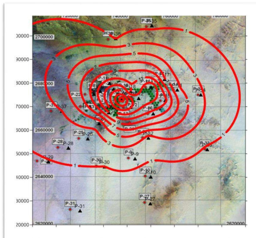
Figure (15) Drawdown in the Deep Aquifer (2010)
