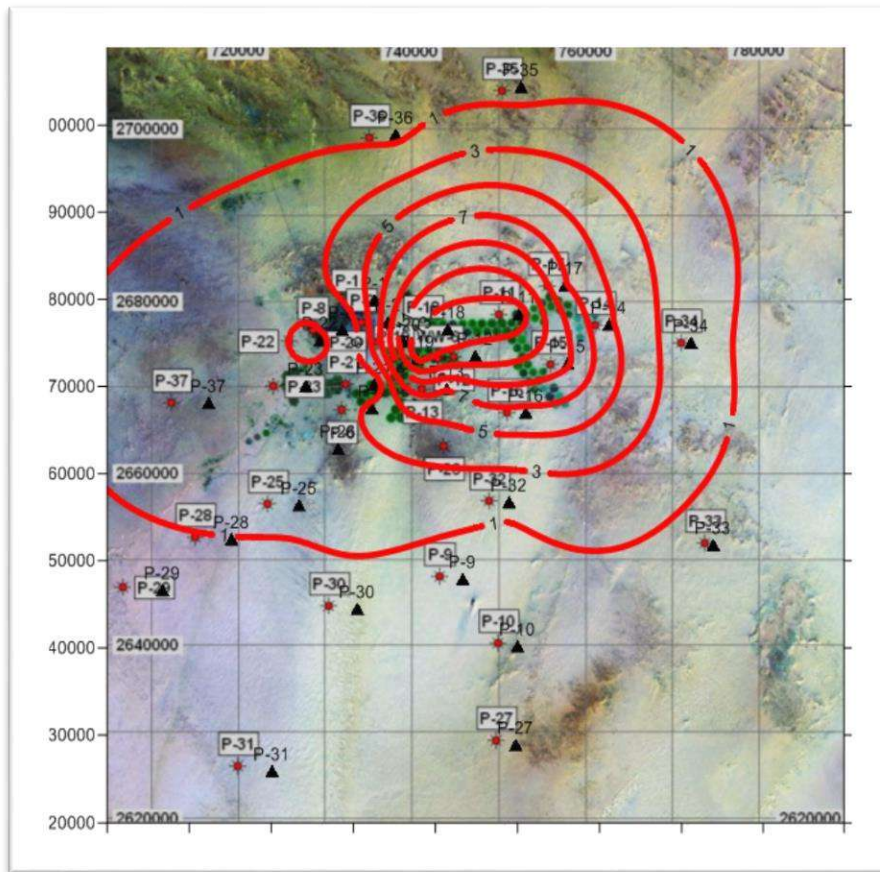
Figure (12) ) Drawdown in the Shallow Aquifer (2000)
