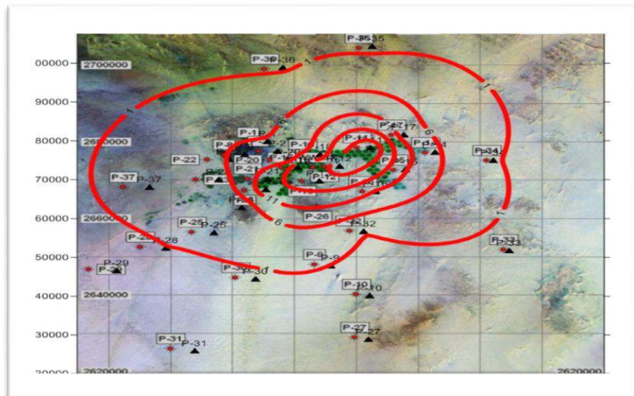
Figure (11) ) Drawdown in the Deep Aquifer (1990)
