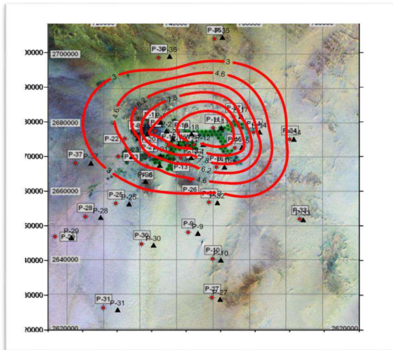
Figure (14) ) Drawdown in the Shallow Aquifer (2010)
