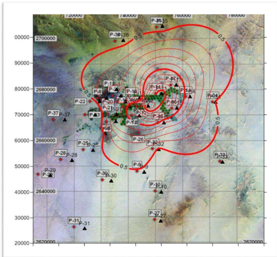
Figure (10) ) Drawdown in the Shallow Aquifer (1990)
