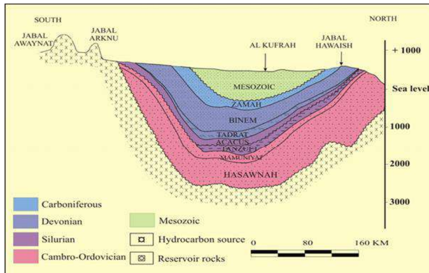
Figure (5) Hydrological section of the north-south Kufra Basin (Palas, 1980)
