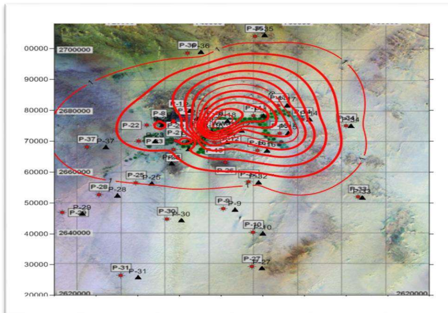
Figure (9) Drawdown in the Deep Aquifer (1980)
