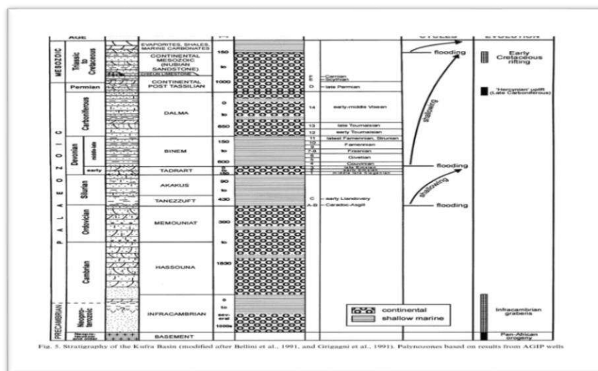
Figure (4) Geological formations in the study area
