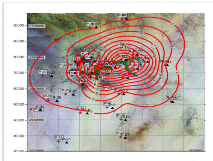
Figure (13) ) Drawdown in the Deep Aquifer (2000)
