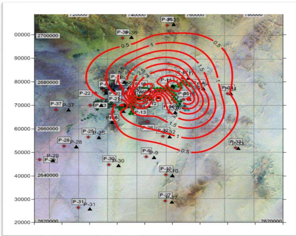
Figure (8) Drawdown in the Shallow Aquifer 1980
