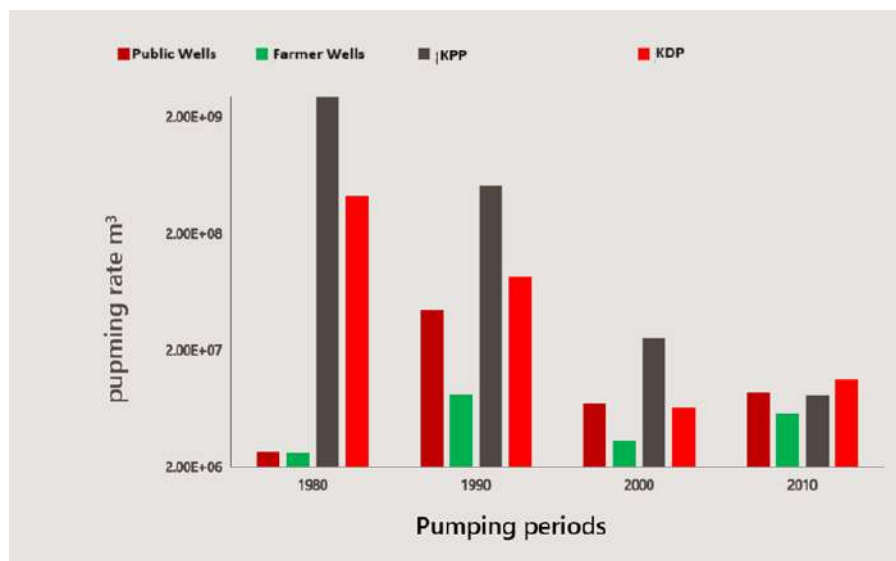
Figure (6) Pumping quantities from strategic projects and citizens' wells
